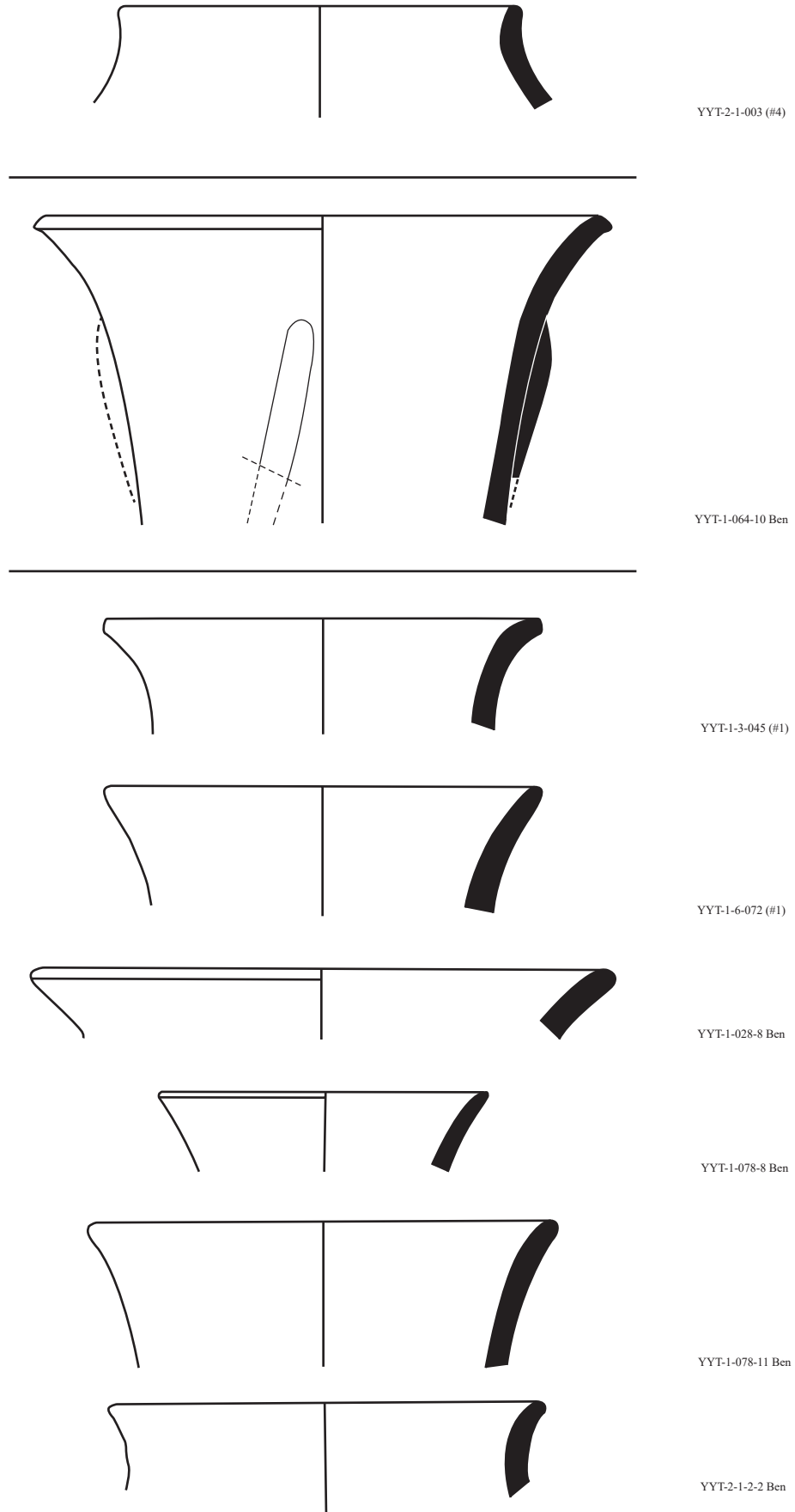
Yeni Yeldeğirmen-tepe - Excavations Neck-jar 1, Neck-jar 2, Neck-jar 3 (M 1:2)
