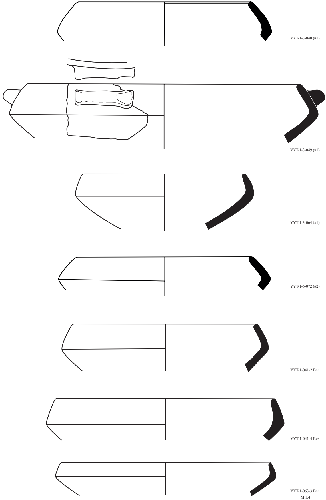
Yeni Yeldeğirmen - Excavations Shallow bowl 1a (M 1:2)
