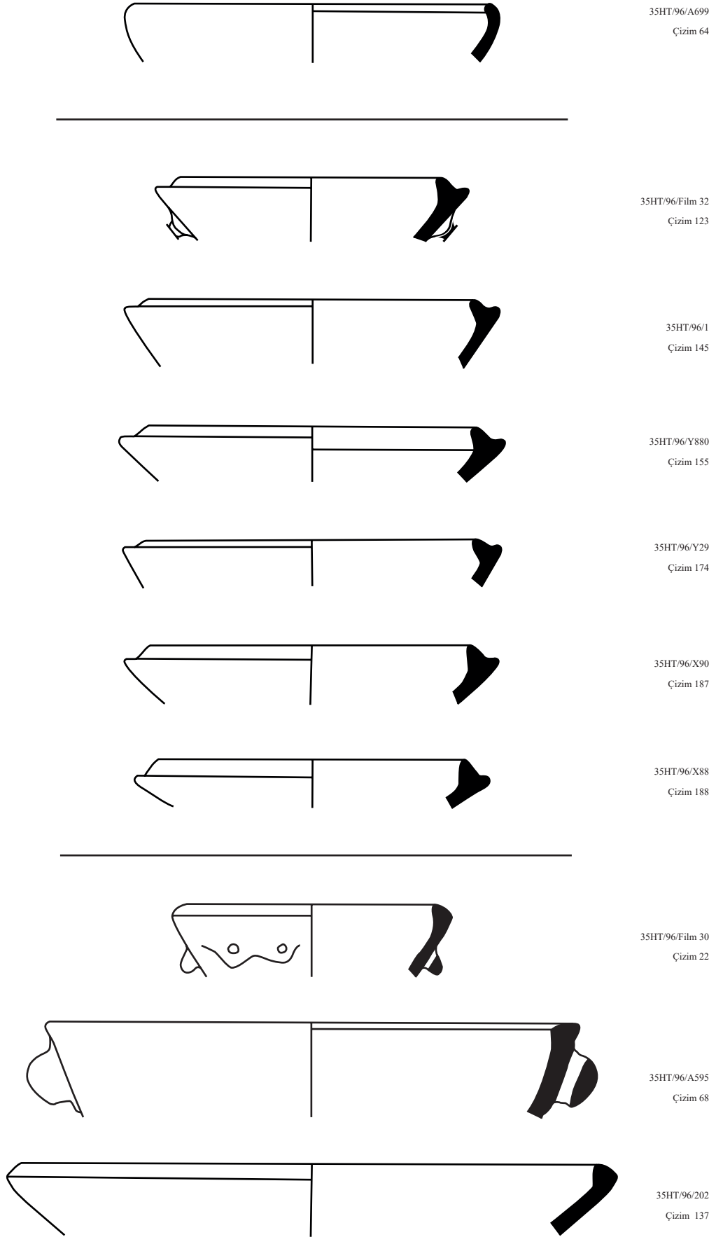
Hüyüktepe - Survey Shallow bowl 4, Shallow bowl 5, Shallow bowl 6a (M 1:2)
